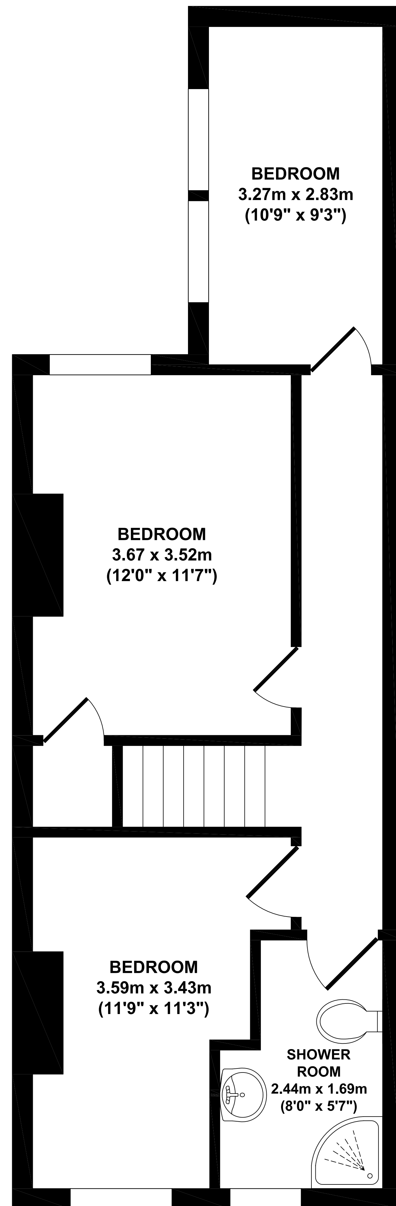
FIRST FLOOR
